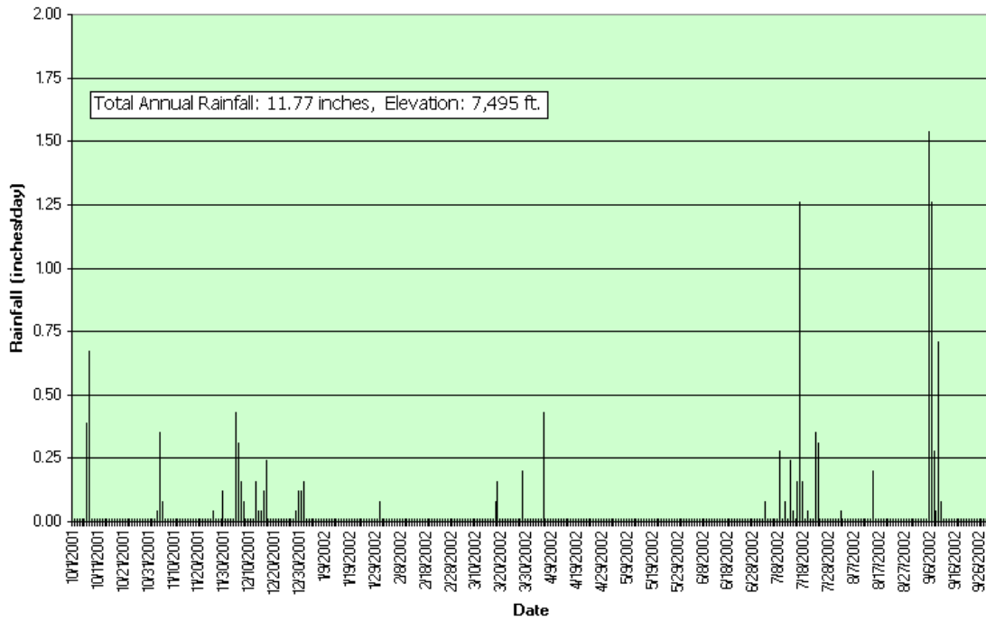
Mt. Union Precipitation Gage No. 5380 Water-Year 2002
