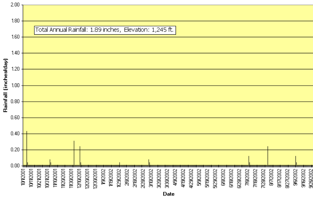
Bender Wash Precipitation Gage No. 6960 Water-Year 2002
