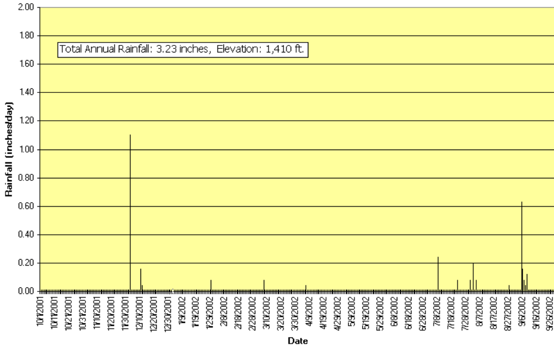
Queen Creek Road Precipitation Gage No. 6610 Water-Year 2002
