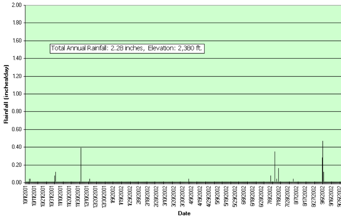
Wickenburg Airport Precipitation Gage No. 7120 Water-Year 2002
