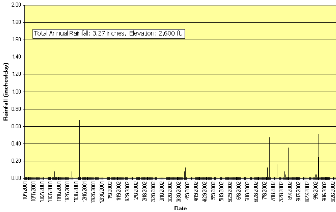
Reata Pass Dam Precipitation Gage No. 4935 Water-Year 2002
