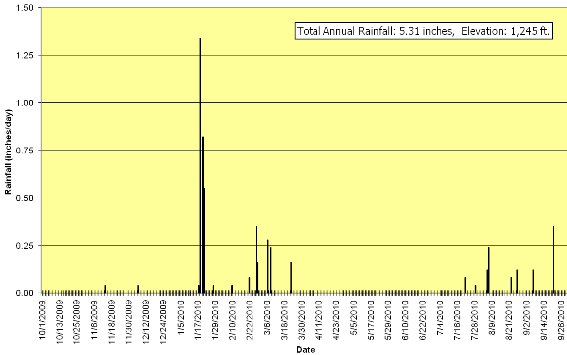
Bender Wash Precipitation Gage No. 6960 Water-Year 2010
