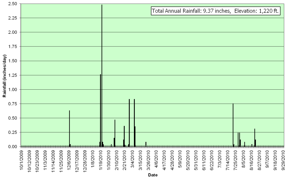
AZ Canal Diversion Channel at 67th Ave. Precipitation Gage No. 5520 Water-Year 2010
