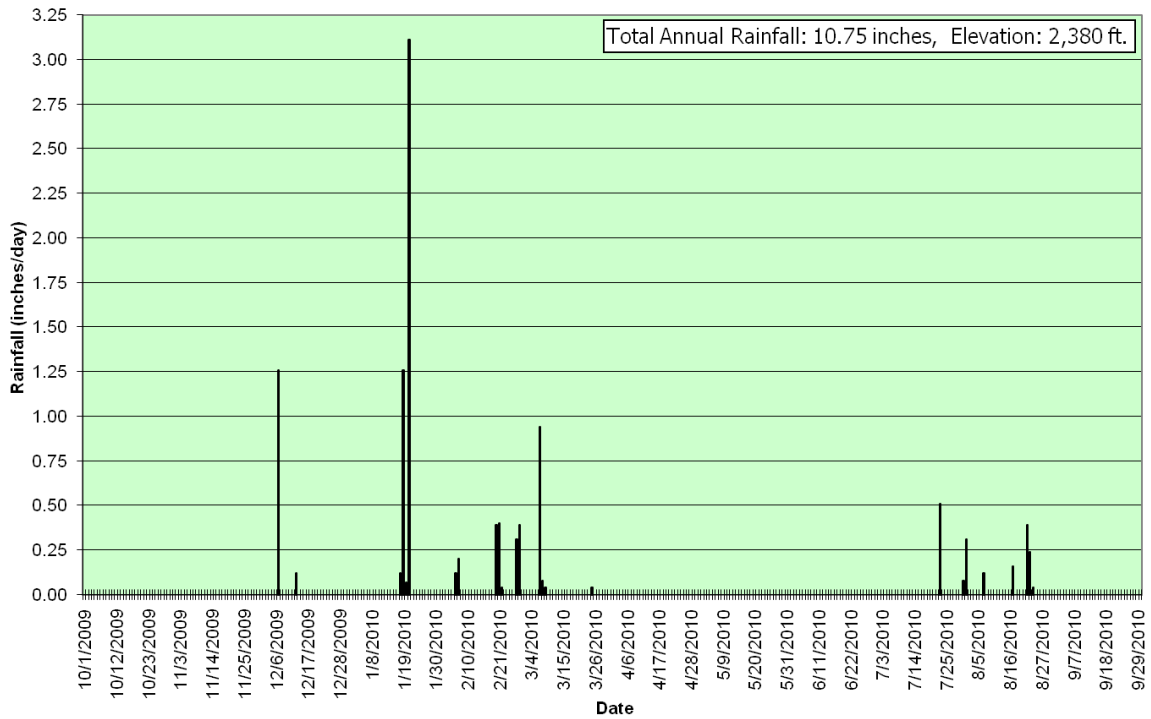
Wickenburg Airport Precipitation Gage No. 7120 Water-Year 2010
