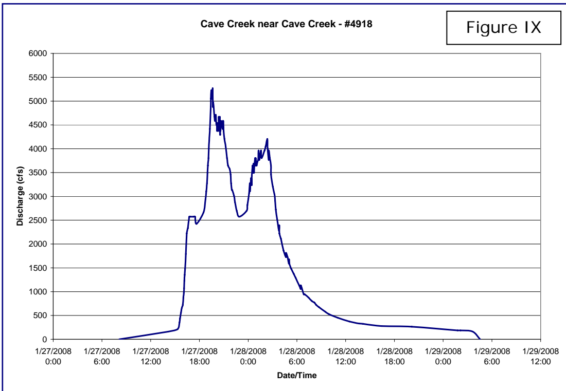
Recorded hydrograph at Cave Creek near Cave Creek, streamgage # 4918, which is approximately 5 miles upstream of Cave Buttes Dam.
