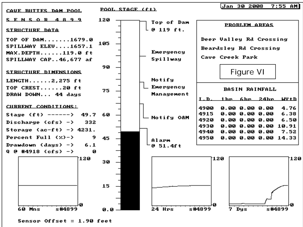
Cave Buttes Dam impoundment information at its peak stage value of 49.7 ft. at 07:55 on January 30th. Although it reached 4,231 acre-feet of storage, it did not reach alarm level (10% full).
