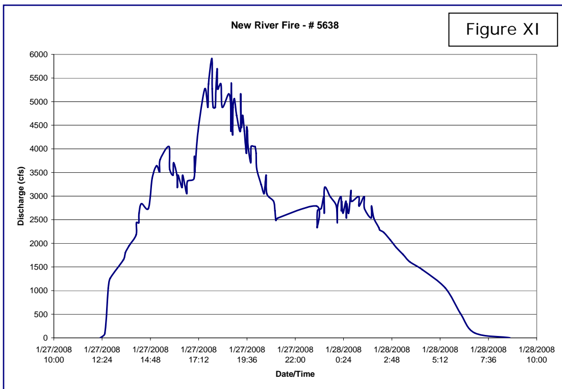
Recorded hydrograph at New River Fire, streamgage # 5638, which is approximately 20 miles upstream of New River Dam.
