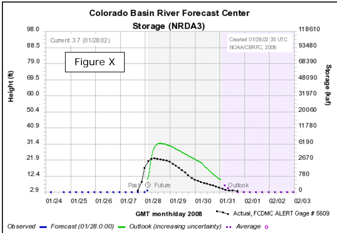
Figure X above shows the forecast inflow hydrograph for New River Dam in green, and the actual recorded hydrograph from FCD Gage #5609 in black. Note that the reservoir height and acre-feet of storage are significantly overestimated and the time of peak storage is late. The predicted hydrograph was generated about 6 hours after flow actually reached the gage. An inflow hydrograph vs. forecast is not presented because the USGS gage on New River near Rock Springs failed during the event.
