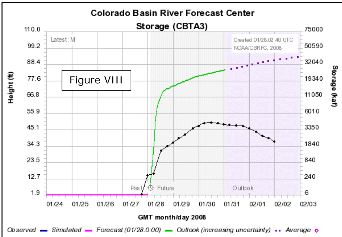
Figure VIII above shows the forecast inflow hydrograph for Cave Buttes Dam in green, and the actual recorded hydrograph from FCD Gage #4899 in black. Note that the reservoir height and acre-feet of storage are significantly overestimated. The predicted hydrograph was generated about 6 hours after flow actually reached the gage.
